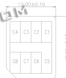
SIM CARD SPEC
